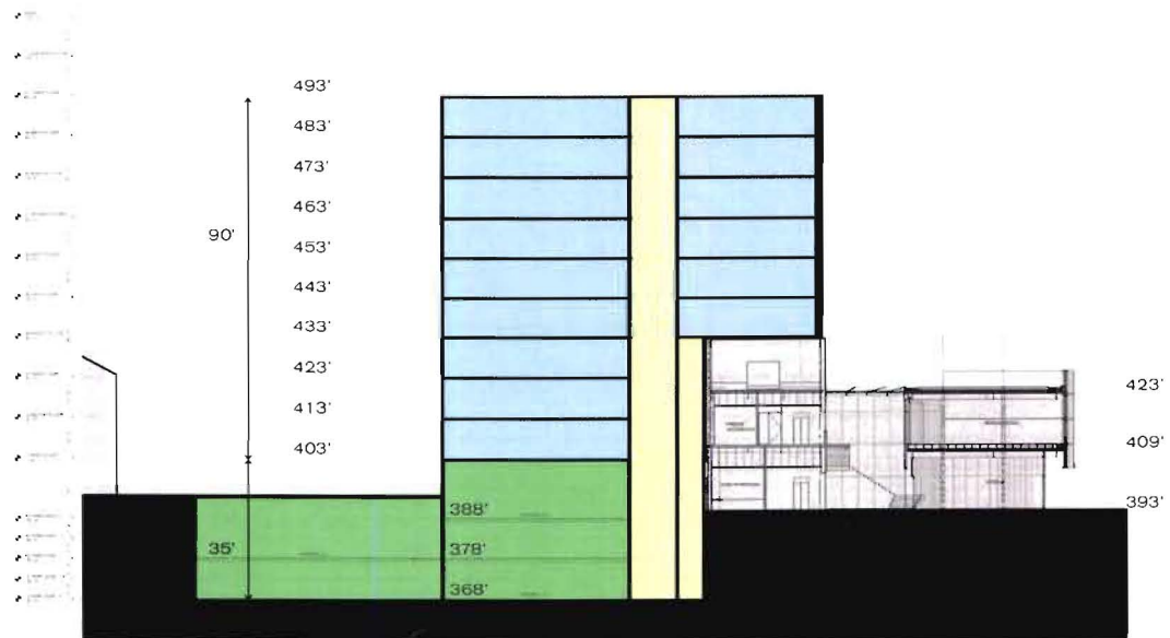
Diagrammatic Building Section 9 Floors
